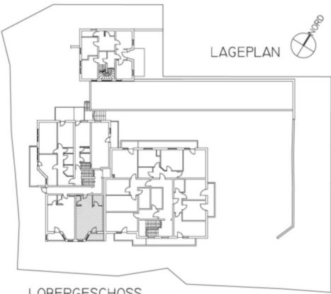
I.OBERGESCHOSS
